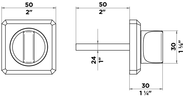
REF. B8E.DWA1C
