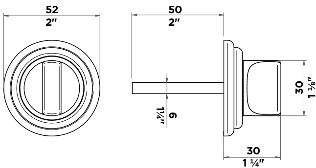
REF. B8B.DWA1C
